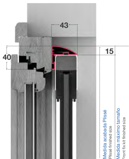
SECC. VERTICAL VERTICAL SECTION
