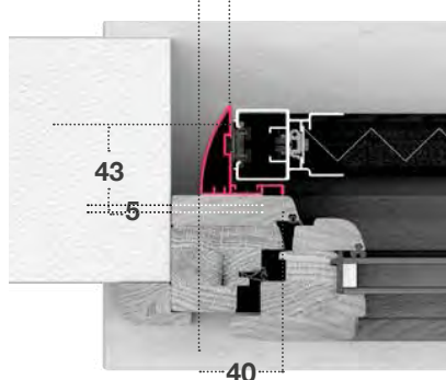
SECC. HORIZONTAL HORIZONTAL SECTION
